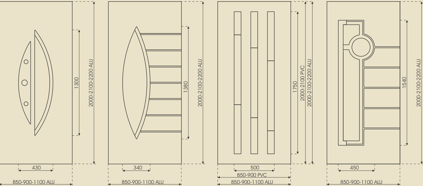
Dimensions and schematic views of decorative panels elite
